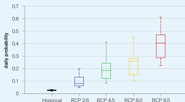
FIGURE 8. Projected changes in daily probability of observing a heat wave in Vietnam under all RCPs. A ‘Heat Wave’ is defined as a period of 3 or more days where the daily temperature is above the long-term 95th percentile of daily mean temperature. 25
