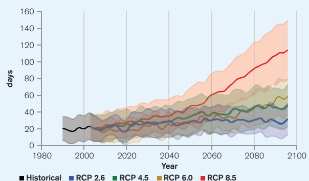
FIGURE 12. Annual average number of hot days (T>35°C) under RCP2.6 (Blue) and RCP8.5 (Red). The values shown represents the median of 30+ GCM model ensemble with the shaded areas showing the 10th–90th percentiles. 66
