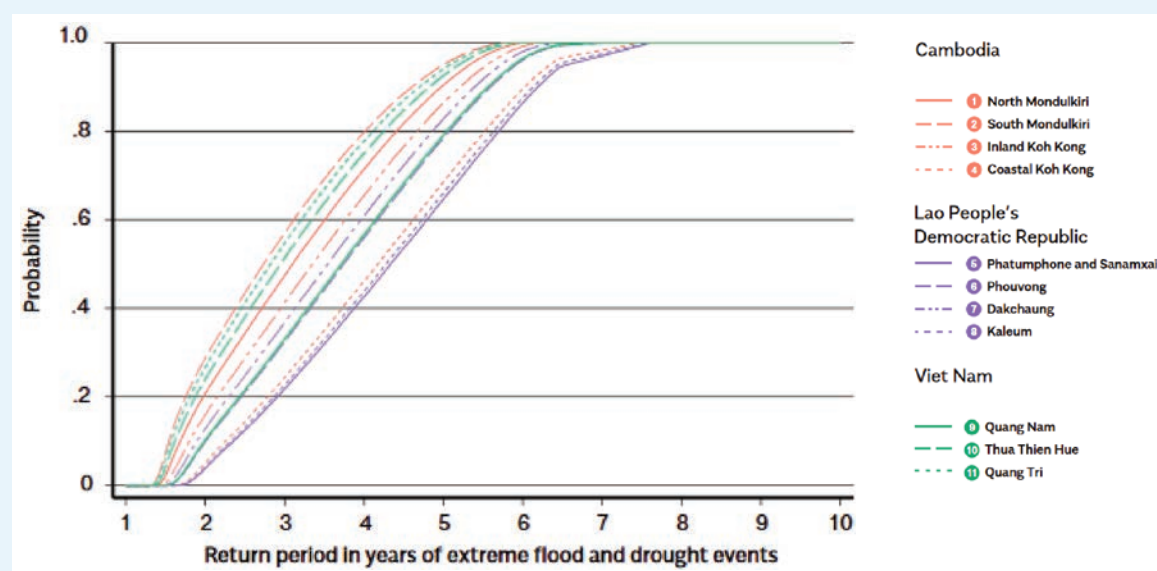
FIGURE 14. Probability of falling into extreme poverty by return period of combined flood and drought events 80
