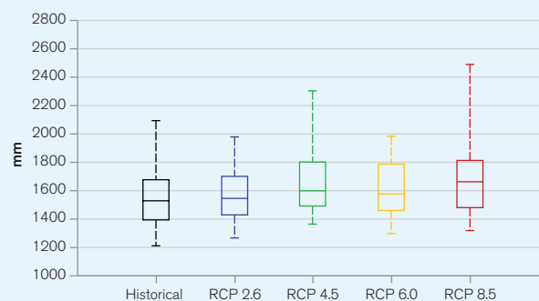
FIGURE 7. Boxplots showing the projected average annual precipitation for Vietnam in the period 2080–2099 17
