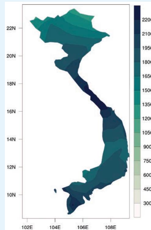
FIGURE 3. Annual mean rainfall (mm) in Vietnam over the period 1901-2019
