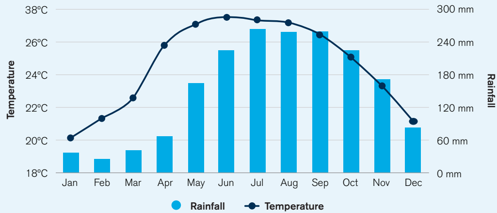
FIGURE 1. Average monthly temperature and rainfall in Vietnam (1991-2019) 5
